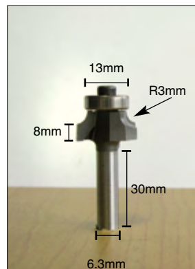
Trimmer Bit for 3mm PVC Edging
