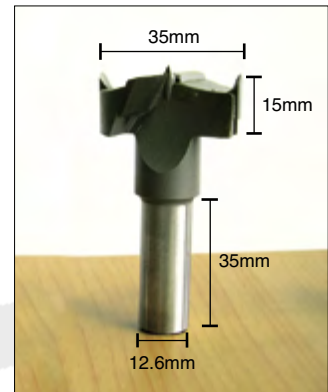
Router Bit for Steel Hinges 35mm Wire Cap
