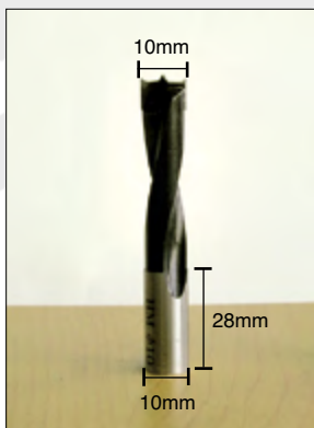
Boring Bit for Minifix-Nylon Nut
