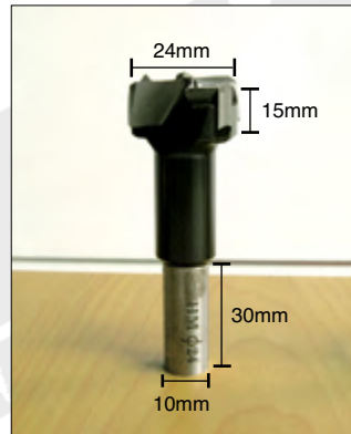
Router Bit for Corner Rack Fitting
