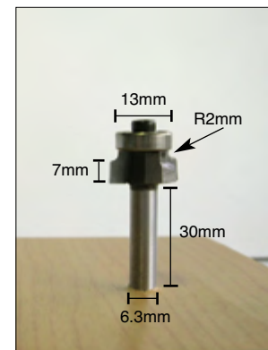
Trimmer Bit for 2mm PVC Edging
