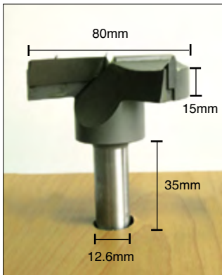
Router Bit for 80mm Wire Cap
