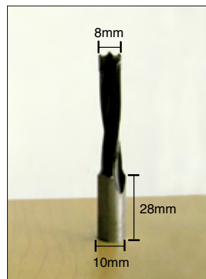
Boring Bit for Minifix-Bolt
