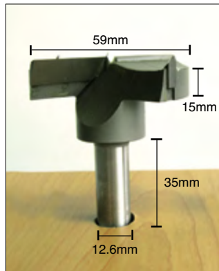
Router Bit for 59mm Wire Cap
