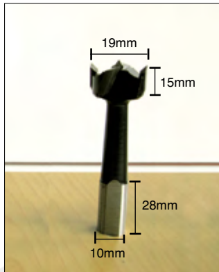
Router Bit for Furniture Lock
