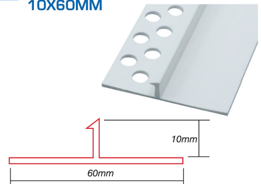
TT4 TRANSITION T-PRIFILE WITH TEETH 10X60MM
