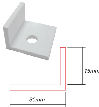
TT2 TRANSITION END L-PROFILE 15X30MM
